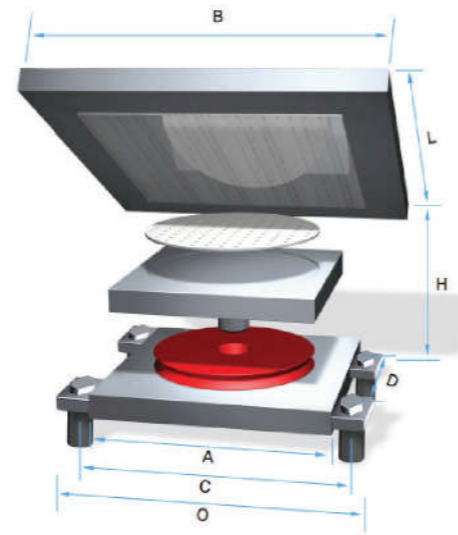
DISK BEARING
