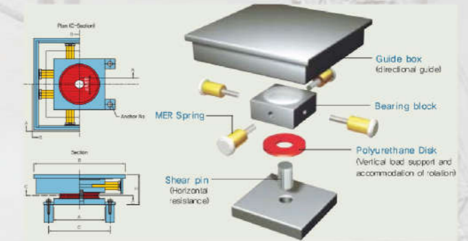
ANTI-EARTHQUAKE BEARING
