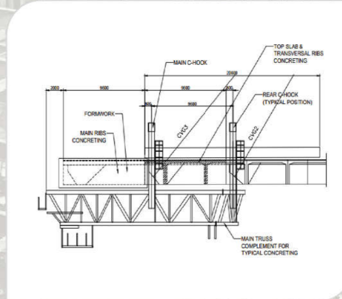
Form traveller
