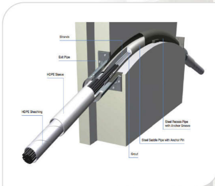
Saddle system
