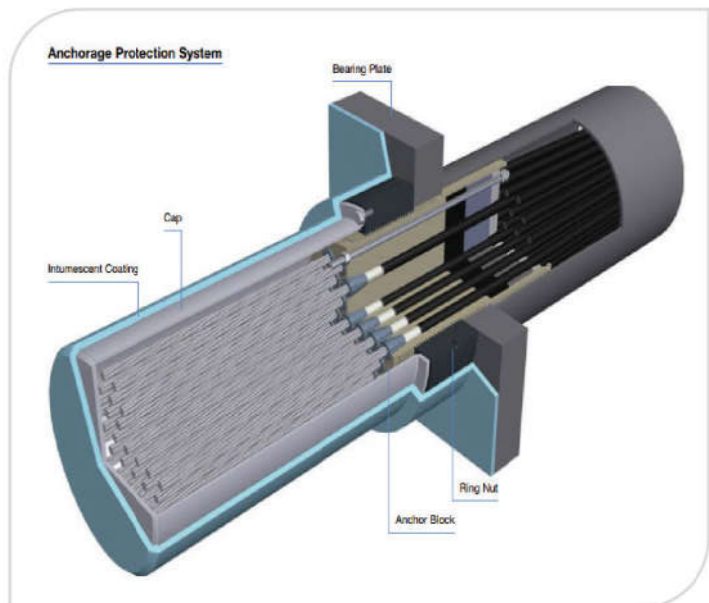
Anchorage for MS cable system
