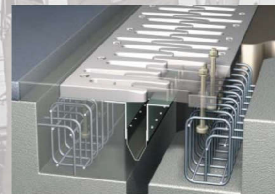
FINGER JOINT
