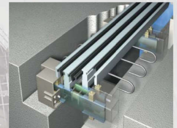
COMPLEX RAIL JOIN
