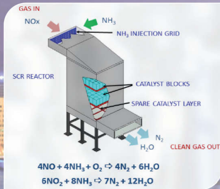
De-NOX SCR technology NSCR technology
