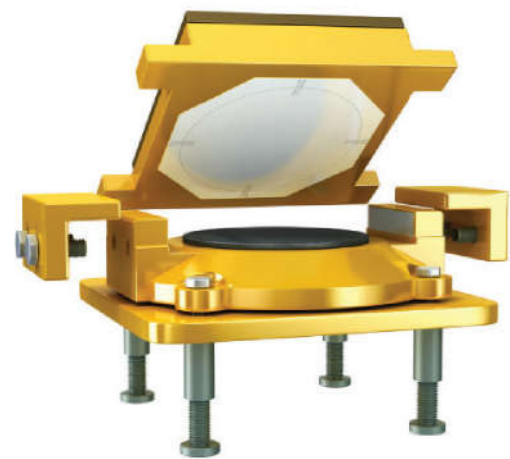
SPHERICAL BEARING
