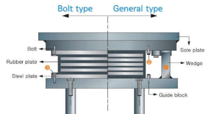
RUBBER BEARING
